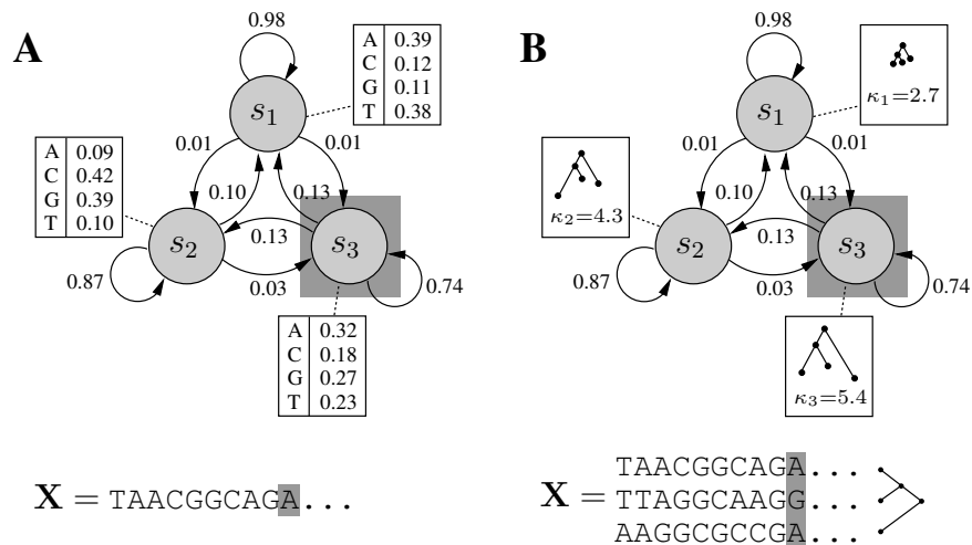
Fig. 1. (A) A 3-state single-sequence HMM, with a multinomial distribution associated with each state (boxed tables). A new state is visited at each time step, according to the indicated transition probabilities (numbers on arcs), and a new character is emitted, according to the probability distribution for that state. The shaded boxes indicate the current state and a newly emitted character, which is appended to the sequence \mathbf{X} . In this example, one state has an A+T rich distribution ( s_1 ), one has a G+C rich distribution ( s_2 ), and one favors purines ( s_3 ). (B) An analogous phylo-HMM. In this case, the multinomial distributions are replaced by phylogenetic models, and at each time step a new column in a multiple alignment \mathbf{X} is emitted. The phylogenetic models include parameters describing the overall shape and size of the tree, as well as the background distribution for characters and the pattern of substitution. For simplicity, the tree parameters are represented graphically, and only one auxiliary parameter is shown.
